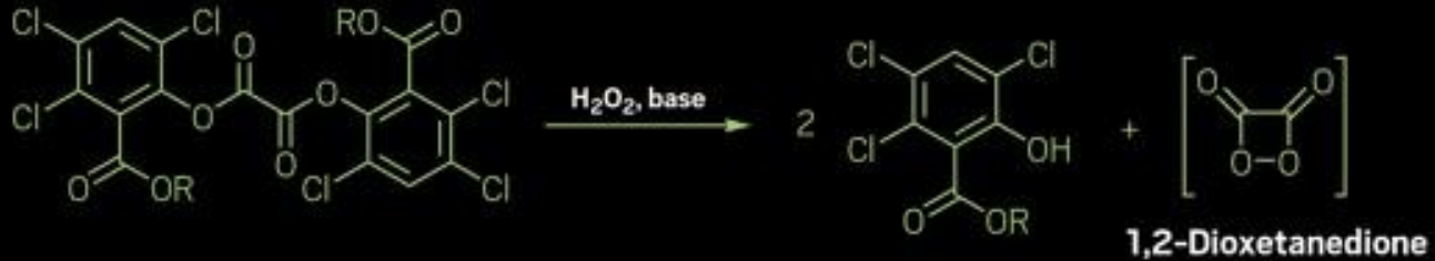
Trichlorosalicylate oxalate ester
